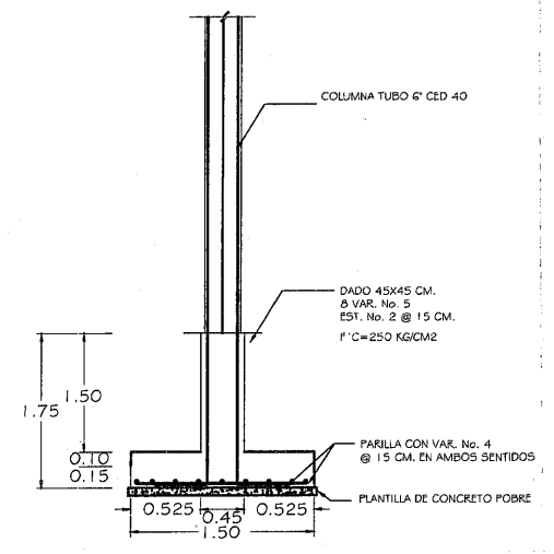
ZAPATA AISLADA "Z-1"
