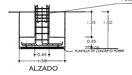
ZAPATA AISLADA "Z-1"
